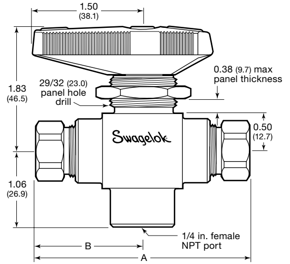
83 Series 3-Way
