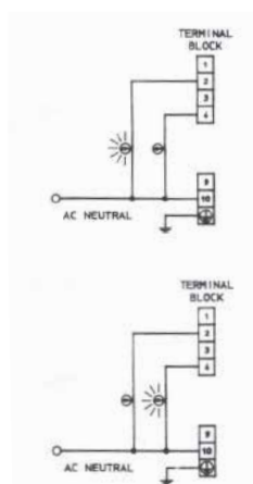
Resulting Lamp Status
