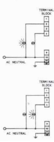
Resulting Lamp Status
