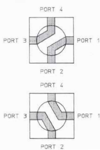
Resulting Valve Stem Position
