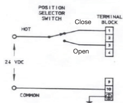
Control Signal Configuration
